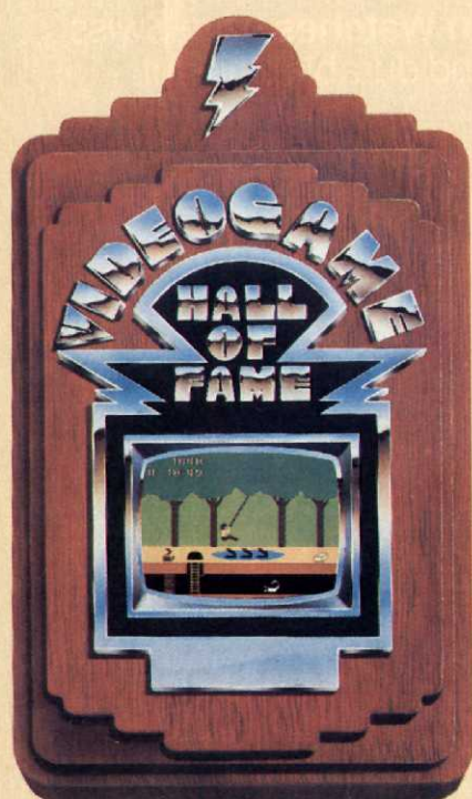
PITFALL (Activision)
