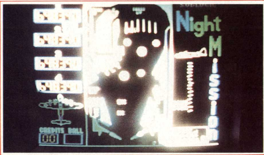
NIGHT MISSION
