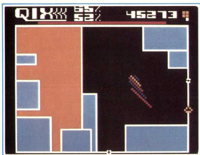
QIX (ATARI 5200)
