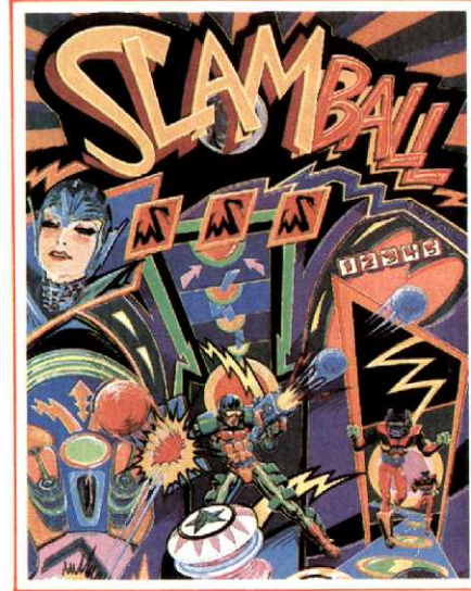
SLAM BALL
