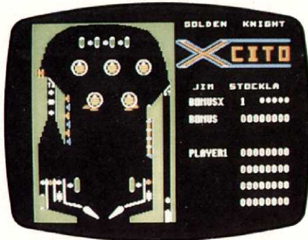
PINBALL PARADISE
