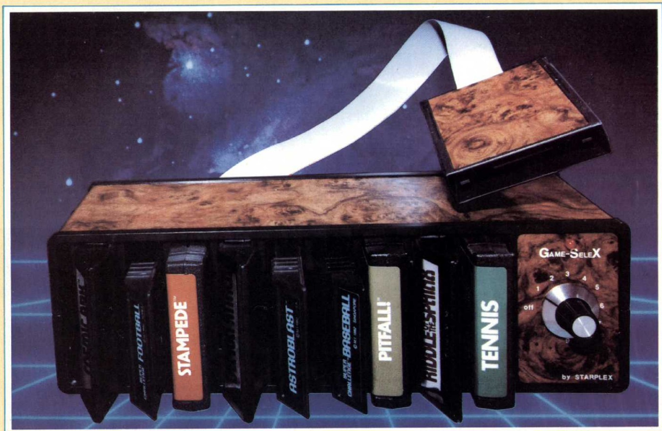
STARPLEX'S GAME-SELEX
