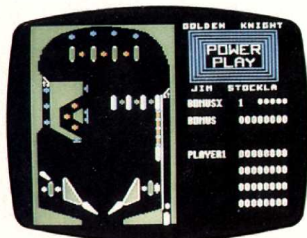
PINBALL PARADISE
