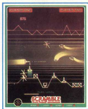
SCRAMBLE (VECTREX)
