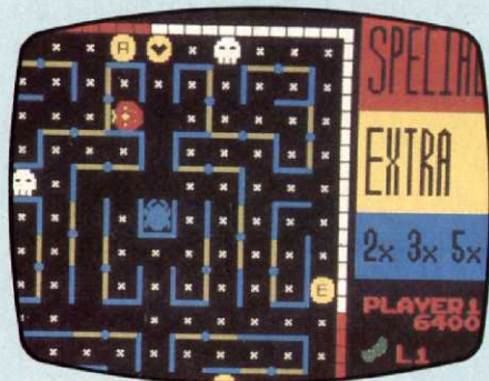
COLECOVISION'S LADYBUG
