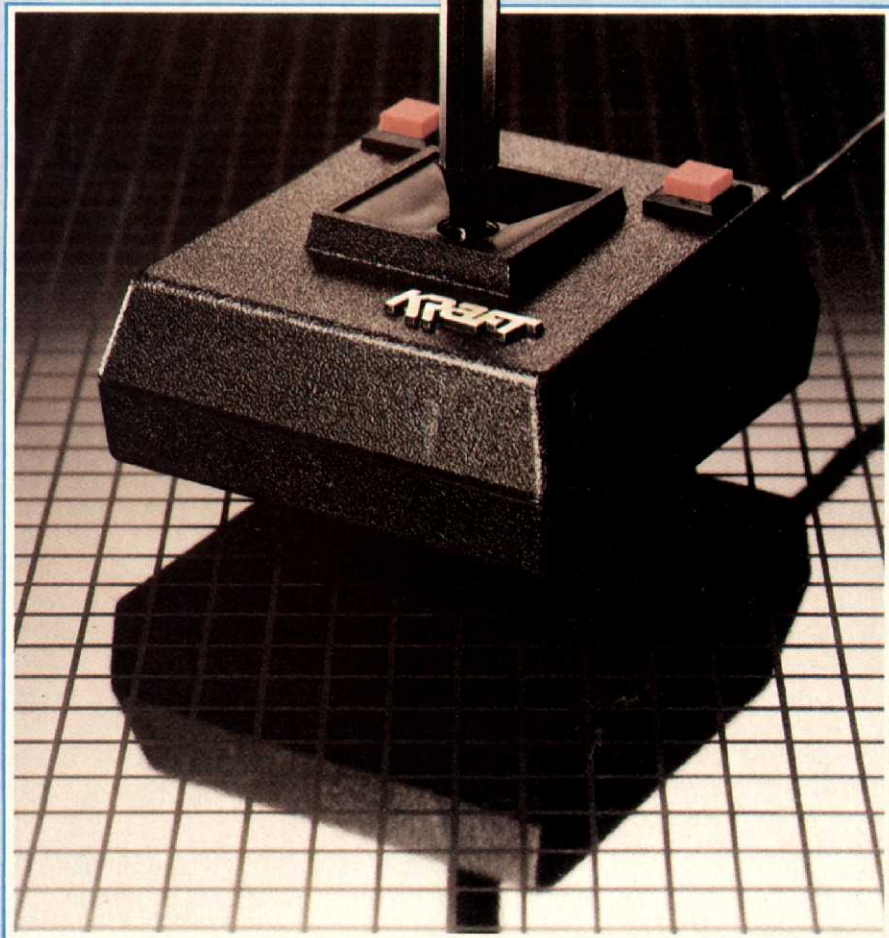
KRAFT'S SWITCH-HITTER
