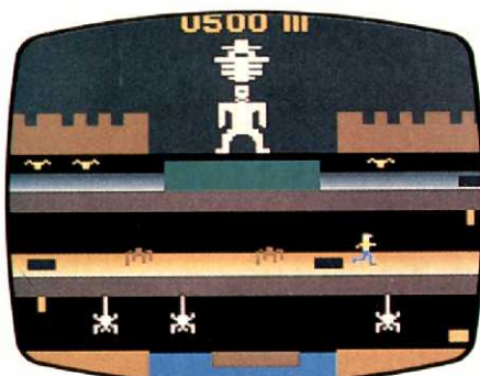
FRANKENSTEIN'S MONSTER
