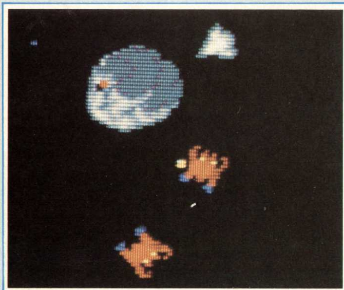
SINISTAR (WILLIAMS)
