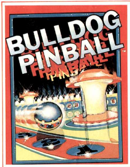
BULLDOG PINBALL
