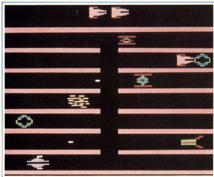
TURMOIL (FOX)
