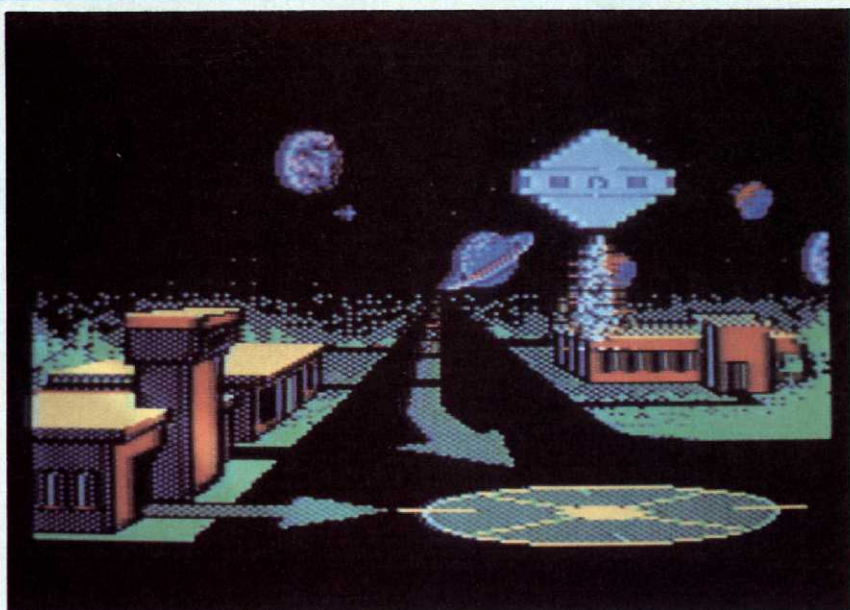
ASTRO CHASE
