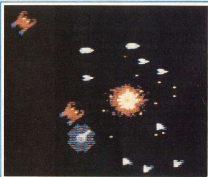
SINISTAR (WILLIAMS)
