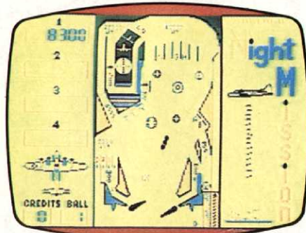
NIGHT MISSION
