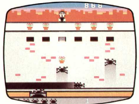
CRACKPOTS (ACTIVISION)
