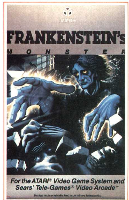
FRANKENSTEIN'S MONSTER
