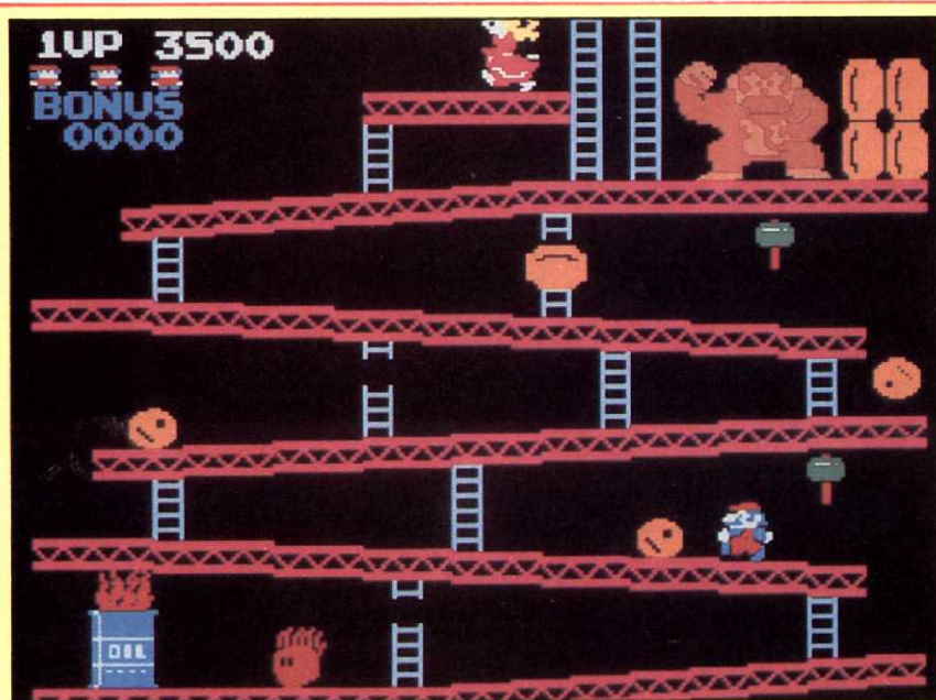
DONKEY KONG
