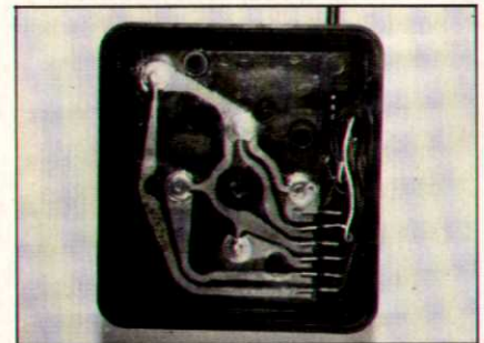
The circuit board in position in the base of the Atari joystick.
